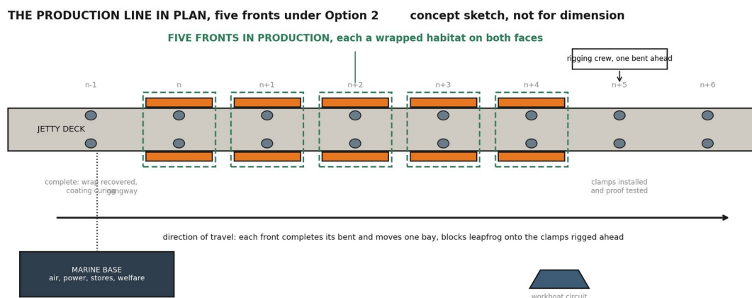
Figure 4. Production line arrangement in plan: fronts in work, the rigging crew one bent ahead, the completed bent curing behind, the marine base serving the fleet. Concept sketch, not for dimension.
